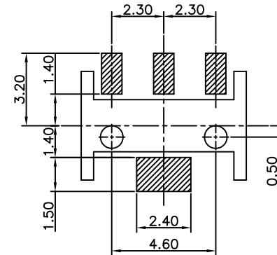
RECOMMEND P.C.BOARD LAYOUT
