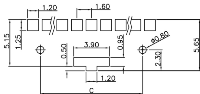
P.C. Board Layout (Tolerance:±0.05)
