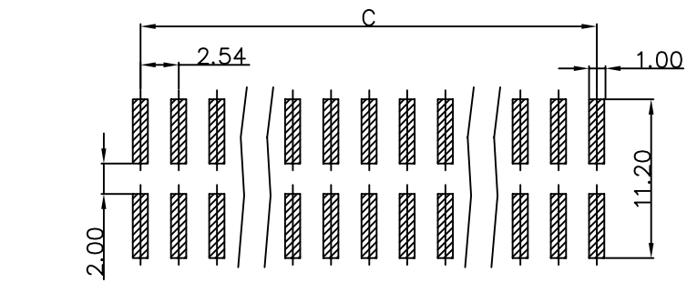
RECOMMEND P.C.B. LAYOUT TOP VIEW
