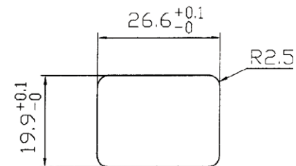
PANEL CUT-OUT
