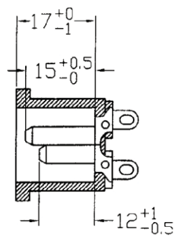
SECTION. AL
