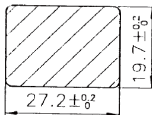
PANEL CUTOUT THICKNESS X mm
