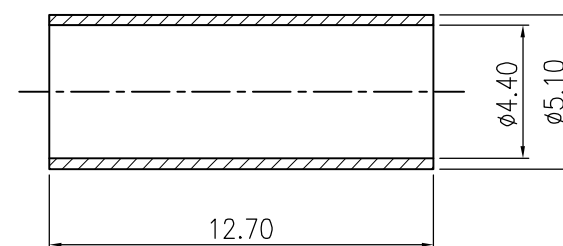
7. FERRULE
