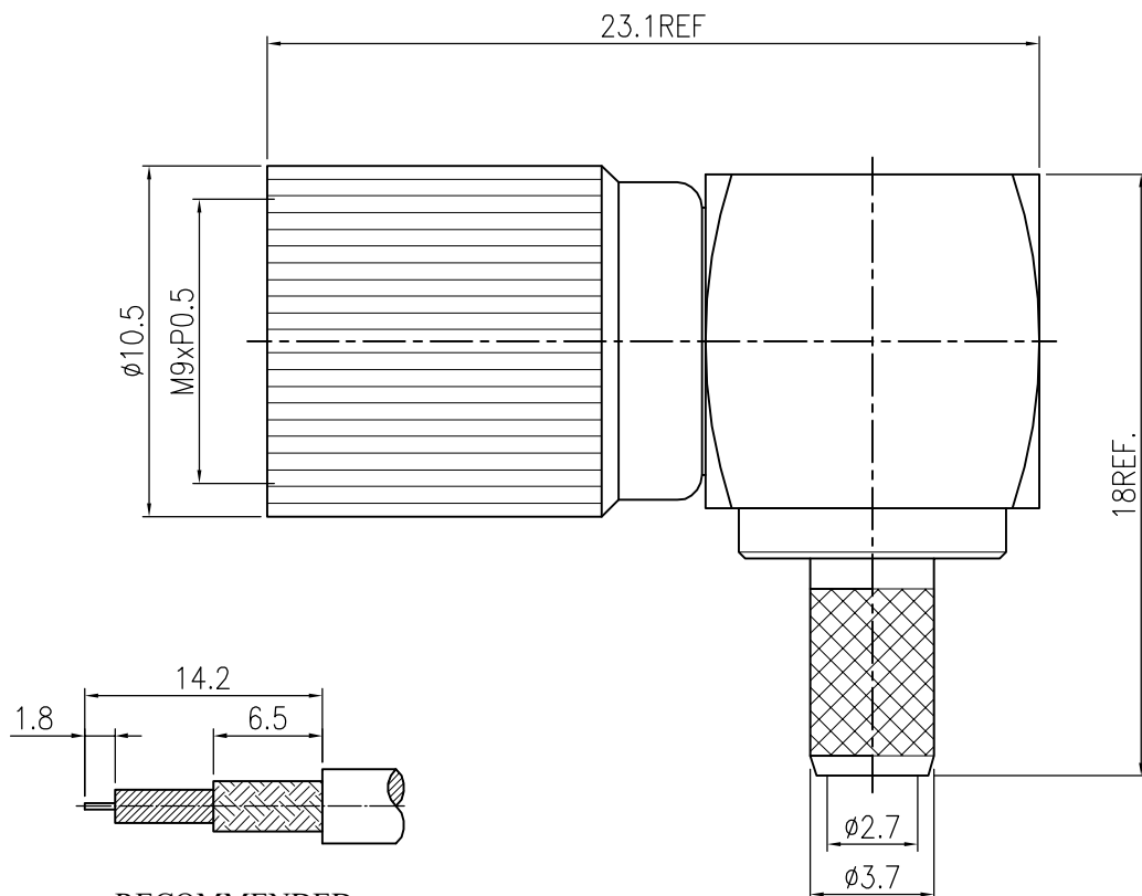
RECOMMENDED CABLE STRIPPING DIM'S
