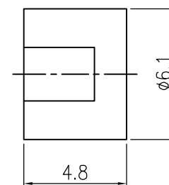
7. FERRULE
