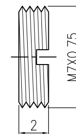
9. SCREW
