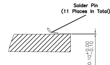
View Of Coplanarity
